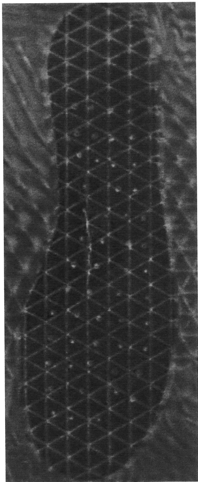
Fig 1. Magnetic field visualization with superimposed magne-view film. The microencapsulated colloidal nickel particles conglomerate in alignment with the magnetic flux lines producing a 2-dimensional image of the pole pattern.
